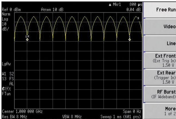
Triangular modulation simplifies spectrum analyzer sweep testing.
